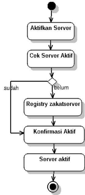
Gambar 2. Activity Diagram Aktifasi Server
