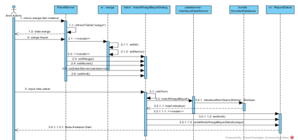
Gambar 8. Sequence Diagram Warga Bayar Zakat
