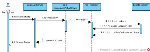
Gambar 6. Sequence Diagram Aktifasi Server
