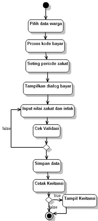
Gambar 4. Activity Diagram Warga Bayar Zakat
