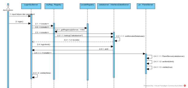
Gambar 7. Sequence Diagram Login
